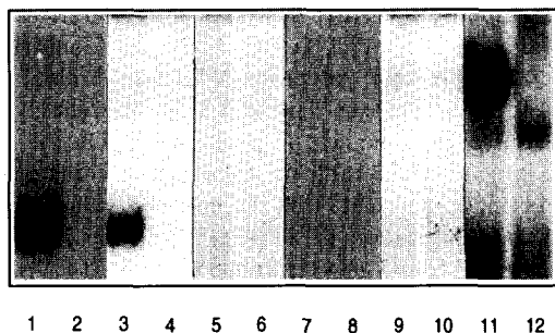
Fig. 2. Activation of STAT factors via gp 130 and the Eg chimera. Untransfected COS-7 cells were stimulated with IL6 (100 B-cell stimulatory factor-2 units/ml) and soluble IL6 receptor (1 μg/ml). Nuclear extracts were prepared. The pattern of STAT activation was analyzed by EMSA and compared to that obtained via the Eg chimera in transfected cells (lanes 1–4). In addition ΔB, a truncated mutant of Eg, was examined with regard to its ability to activate STAT factors (lanes 7–10). As a positive control for STAT5A activation another chimeric receptor consisting of the truncated Eg chimera and the YLVLD tyrosine motif (Y343 of the erythropoietin receptor) was created. Y343 is known to be crucial for STAT5 activation via the erythropoietin receptor. COS-7 cells were transfected with Eg-YLVLD. Nuclear extracts were prepared after stimulation with erythropoietin (7 U/ml) and analyzed by EMSA (lanes 11,12).
